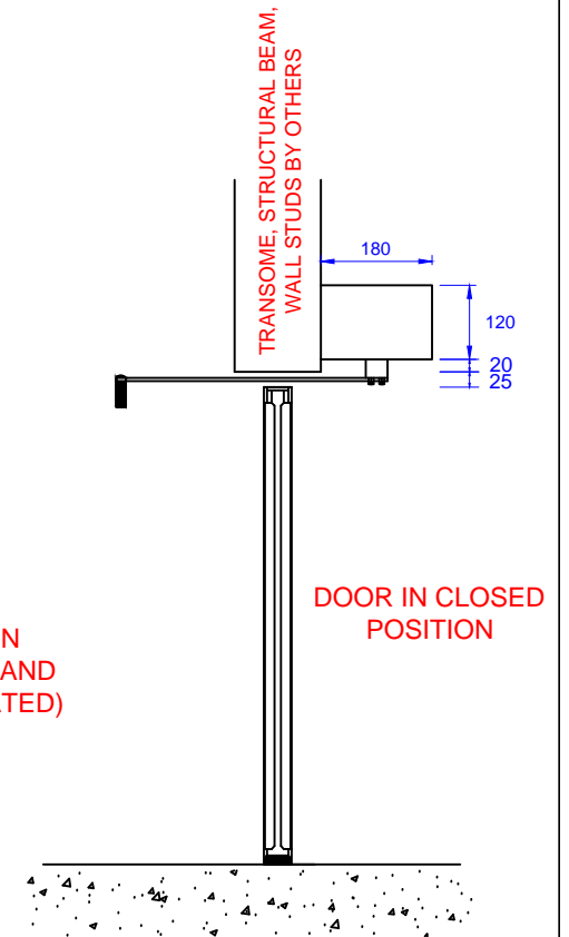
SECTION "A"
