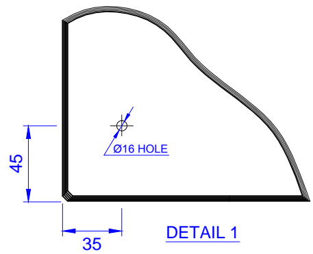
LEADING EDGE BOTTOM CORNER OF DOOR NO.1
